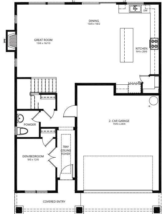
MAIN FLOOR - 1002 SF
