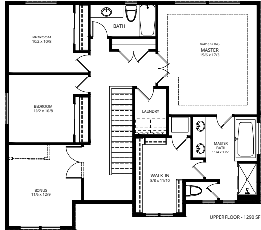
Lot 19 - elevation / floor plan drawings
